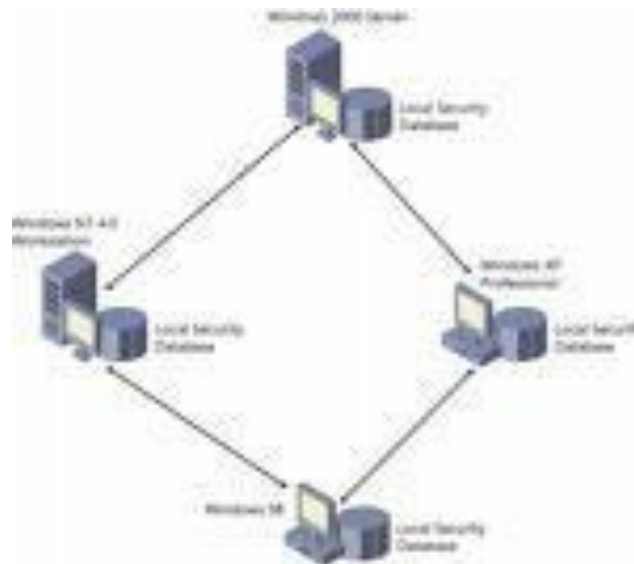
[Peer-Peer architecture]
